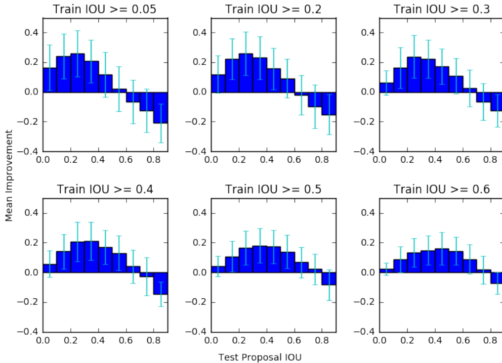
Figure 4.2: Test proposal IOU plotted against mean improvement from BBR. Each bar shows the expected prediction improvement based on initial proposal IOU. Error bars show standard deviation to demonstrate expected variation.
